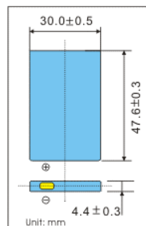
BATTERY DIMENSION
