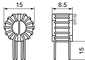
Fig. 22 Choke dimensions (Tokin SC-02-10GS)
