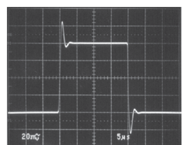
Small-Signal Response
