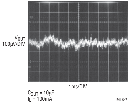
LT1761-5 10Hz to 100kHz Output Noise C_{\text{BY}} = 1000\text{pF}
