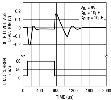
LT1761-5 Transient Response C_{\text{BY}} = 0
