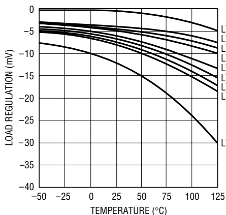
Load Regulation \Delta I_L = 1mA \text{ to } 50mA
