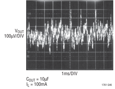
LT1761-5 10Hz to 100kHz Output Noise C_{\text{BY}} = 100\text{pF}
