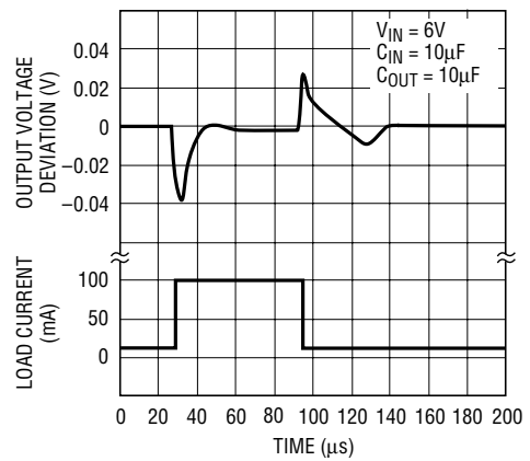
LT1761-5 Transient Response C_{\text{BY}} = 0.01\mu\text{F}
