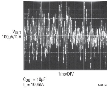
LT1761-5 10Hz to 100kHz Output Noise C_{\text{BY}} = 0
