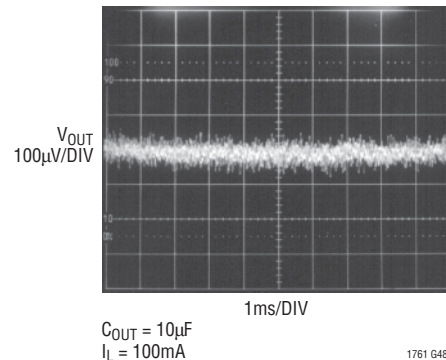
LT1761-5 10Hz to 100kHz Output Noise C_{\text{BY}} = 0.01\mu\text{F}
