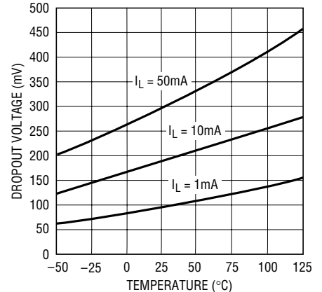
Dropout Voltage
