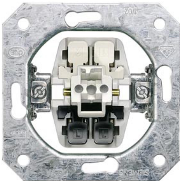
DELTA SWITCH INSERT FM INTERMEDIATE SWITCH 10A 250V
