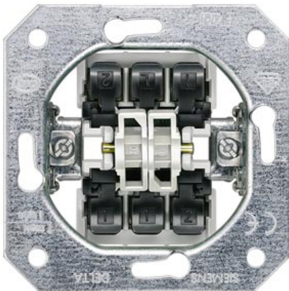
DELTA SWITCH INSERT FM DOPPEL-2-WAY SWITCH 10A 250V
