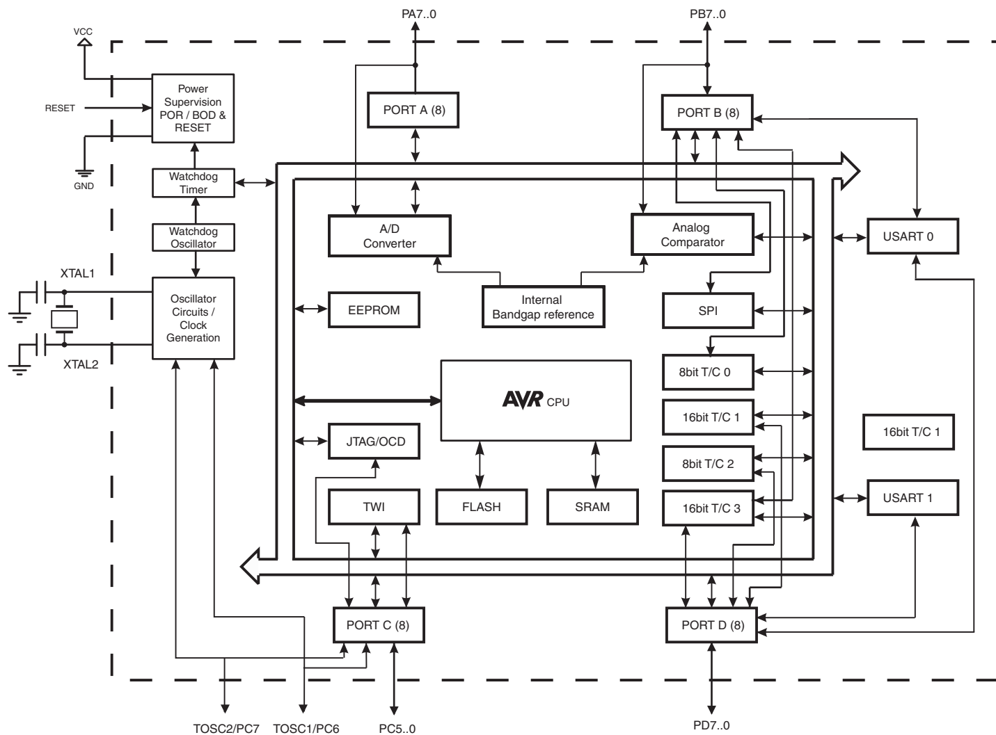
Figure 2-1. Block Diagram
