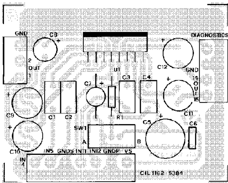
Figure 7. P.C. Board and Component Layout of the fig.4
