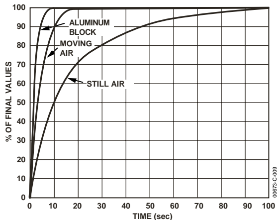
Figure 10. Response Time
