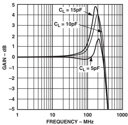
TPC 7. Small Signal Frequency Response for Various C_{LOAD} , V_{OUT} = 500\text{ mV p-p} , V_S = \pm 5\text{ V} , G = +1
