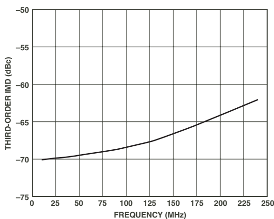
TPC 17. Third-Order Intermodulation Distortion vs. Frequency for a 2 V p-p Composite Signal into R_L = 150\ \Omega ( A_V = 10\ dB , at 5 V Supplies)
