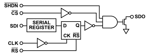
Figure 50. Detailed SDO Output Schematic of the AD8403
