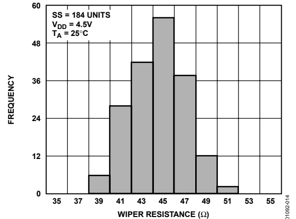
Figure 14. 50 kΩ Wiper-Contact-Resistance Histogram
