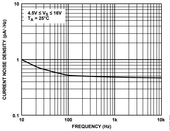
Figure 6. Current Noise Density vs. Frequency
