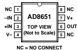
Figure 3. 8-Lead SOIC (R-8)
