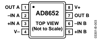
Figure 2. 8-Lead MSOP (RM-8)
