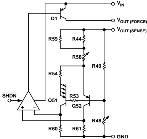
Figure 40. Simplified Schematic
