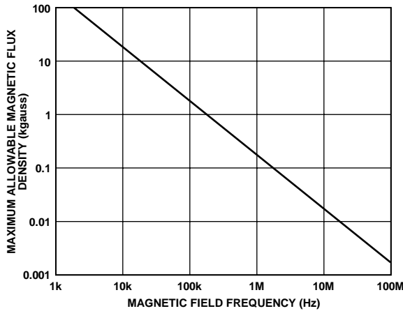
Figure 13. Maximum Allowable External Magnetic Flux Density
