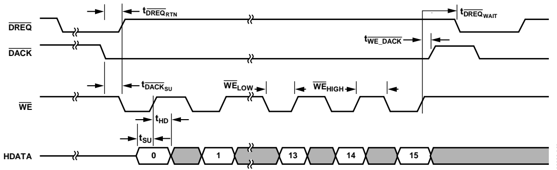
Figure 14. Burst Write Cycle for \overline{DREQ} /DMA Mode for Assigned DMA Channel (EDMOD0/EDMOD1[14:1] Programmed to a Value of 0000)
