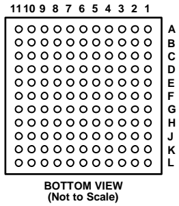
Figure 30. 121-Ball Pin Configuration
