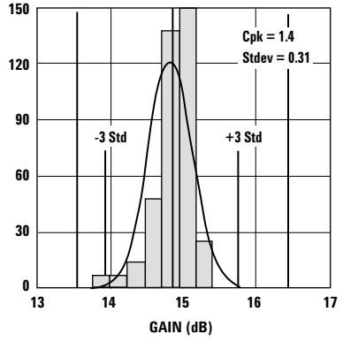
Figure 4. Gain LSL = 13.5, Nominal = 14.8, USL = 16.5.
