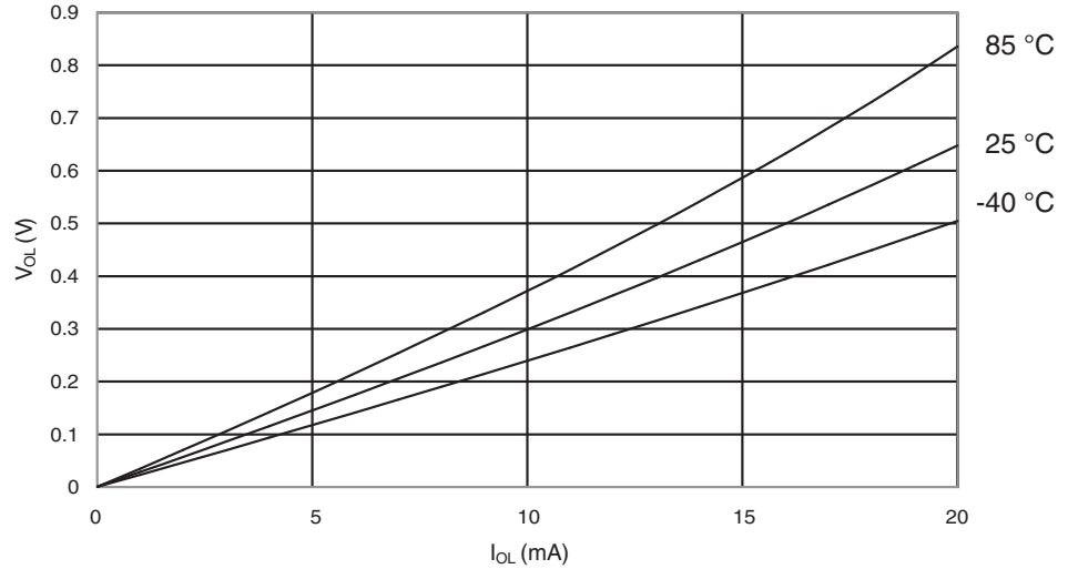
Figure 26-21. I/O Pin Output Voltage vs. Sink Current ( V_{CC} = 3V ).
