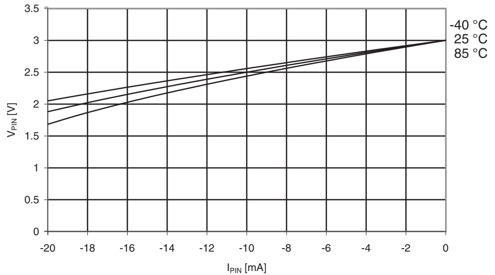
Figure 34-22. I/O Pin Output Voltage vs. Source Current
