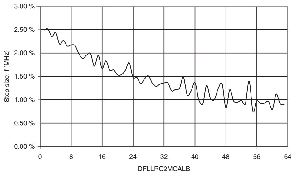
Figure 34-39. Internal 2 MHz Oscillator CALB Calibration Step Size
