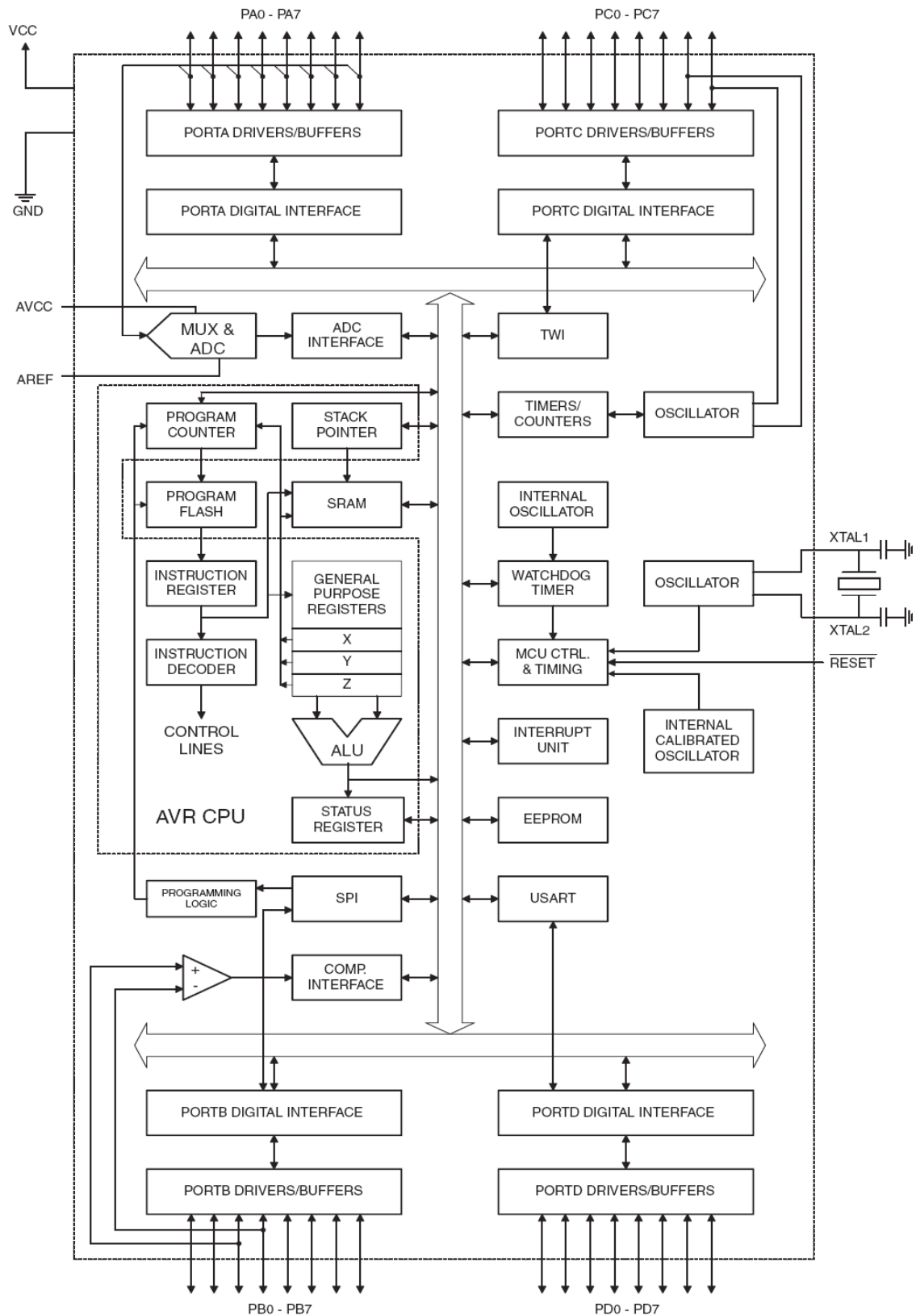
Figure 2. Block Diagram
