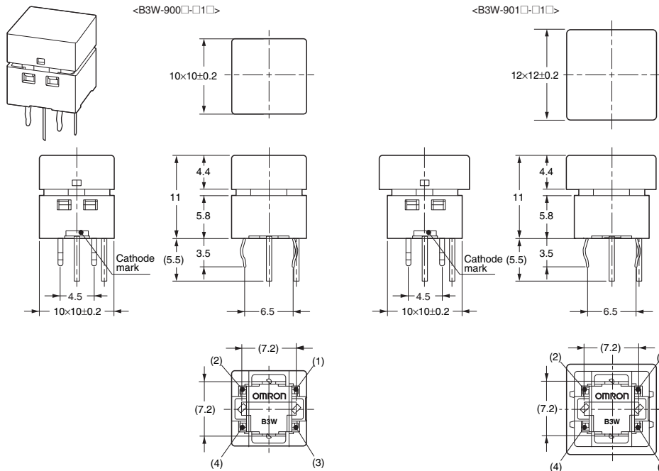
Terminal Arrangement/ Internal Connections (Top View)
