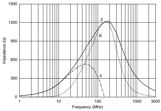
BLM03AG102SN1
