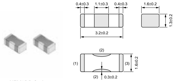
NFM3DP Series
