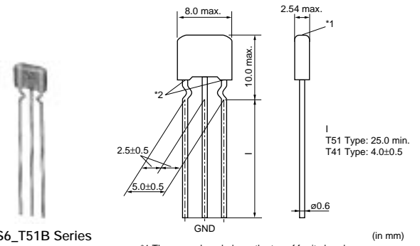
DSS6_T51B Series Incrimp Type
