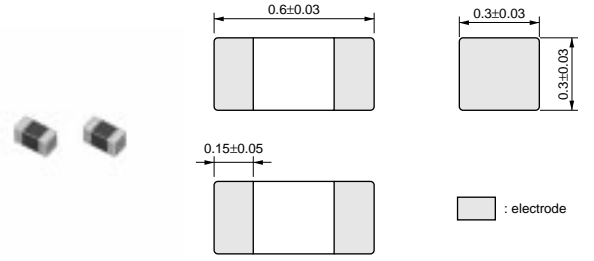
BLM03A Series
