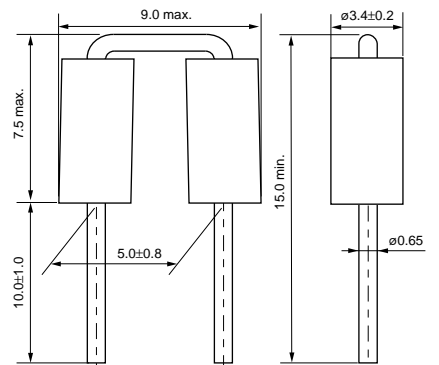
BL02RN2R1M2B
