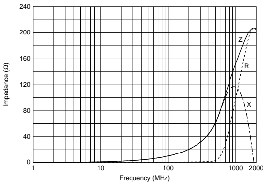
BLM15BA100SN1
