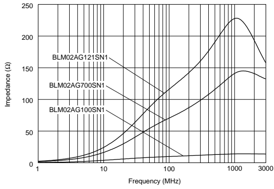
BLM02A Series
