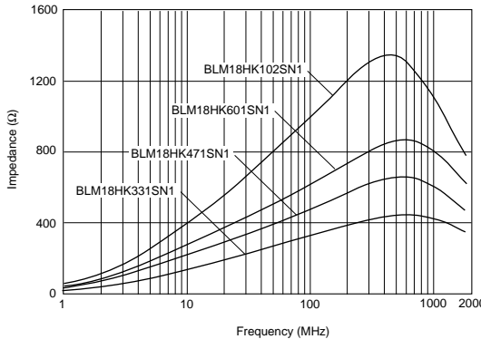
BLM18HK Series
