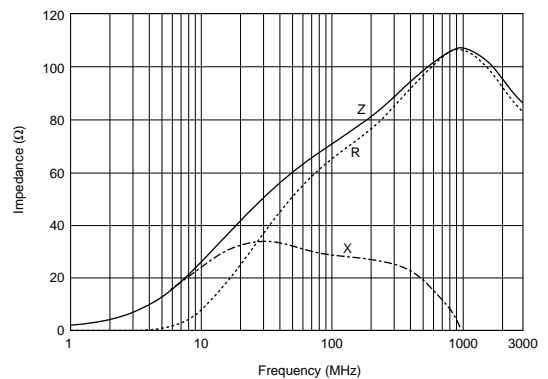
BLM03AG700SN1
