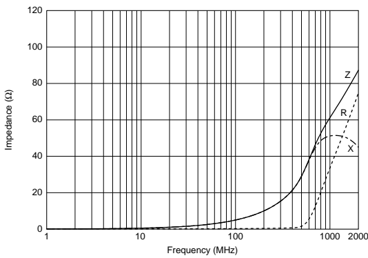
BLM15BA050SN1
