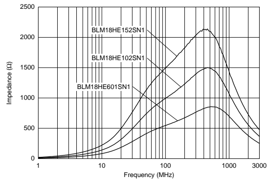
BLM18HE Series
