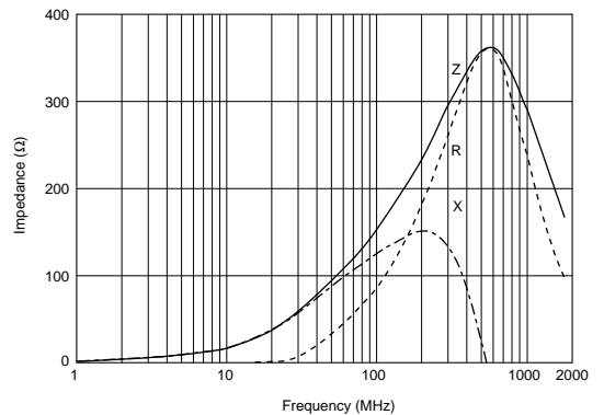
BLM18BD151SN1
