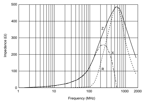
BLM18BB121SN1
