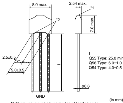
DSS6_Q55B Series Straight Type
