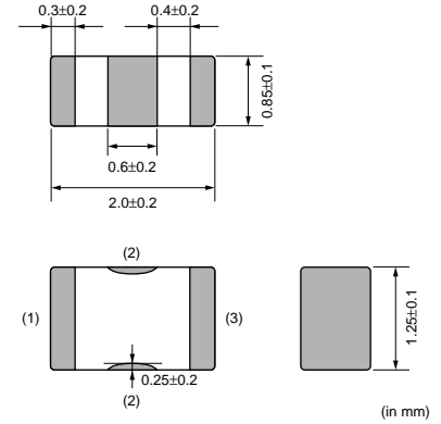
NFL21S Series
