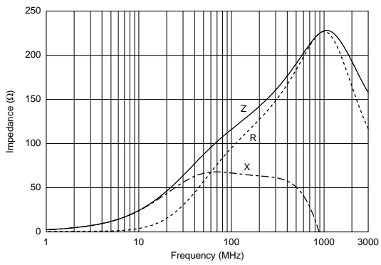
BLM02AG121SN1
