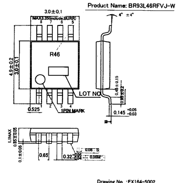
Fig4-(f) PHYSICAL DIMENSION TSSOP-B8J (BR93L46RFVJ-W)
