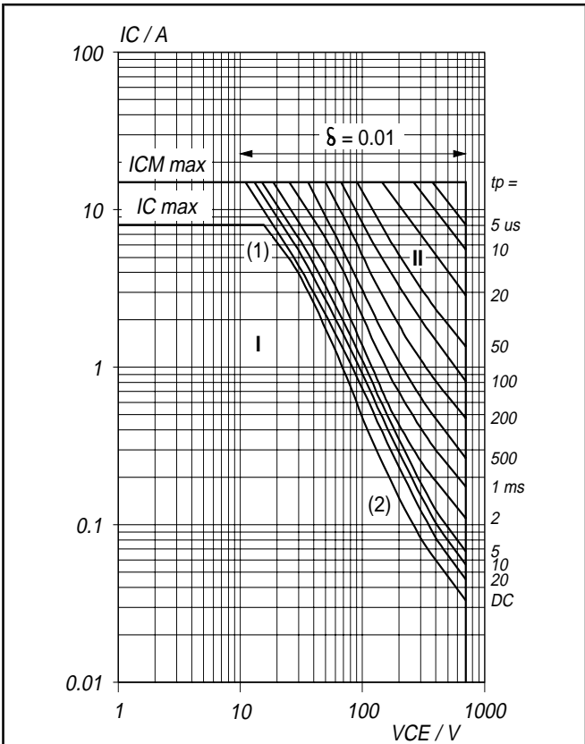
Fig. 13. Forward bias safe operating area. T_{mb} = 25^\circ C (1) P_{tot\ max} line. (2) Second-breakdown limits (independent of temperature). I Region of DC operation. II Extension for repetitive pulse operation.
