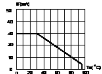
FIG.5 MAXIMUM FORWARD CURRENT VS. AMBIENT TEMPERATURE (Tamb=105 °C)
