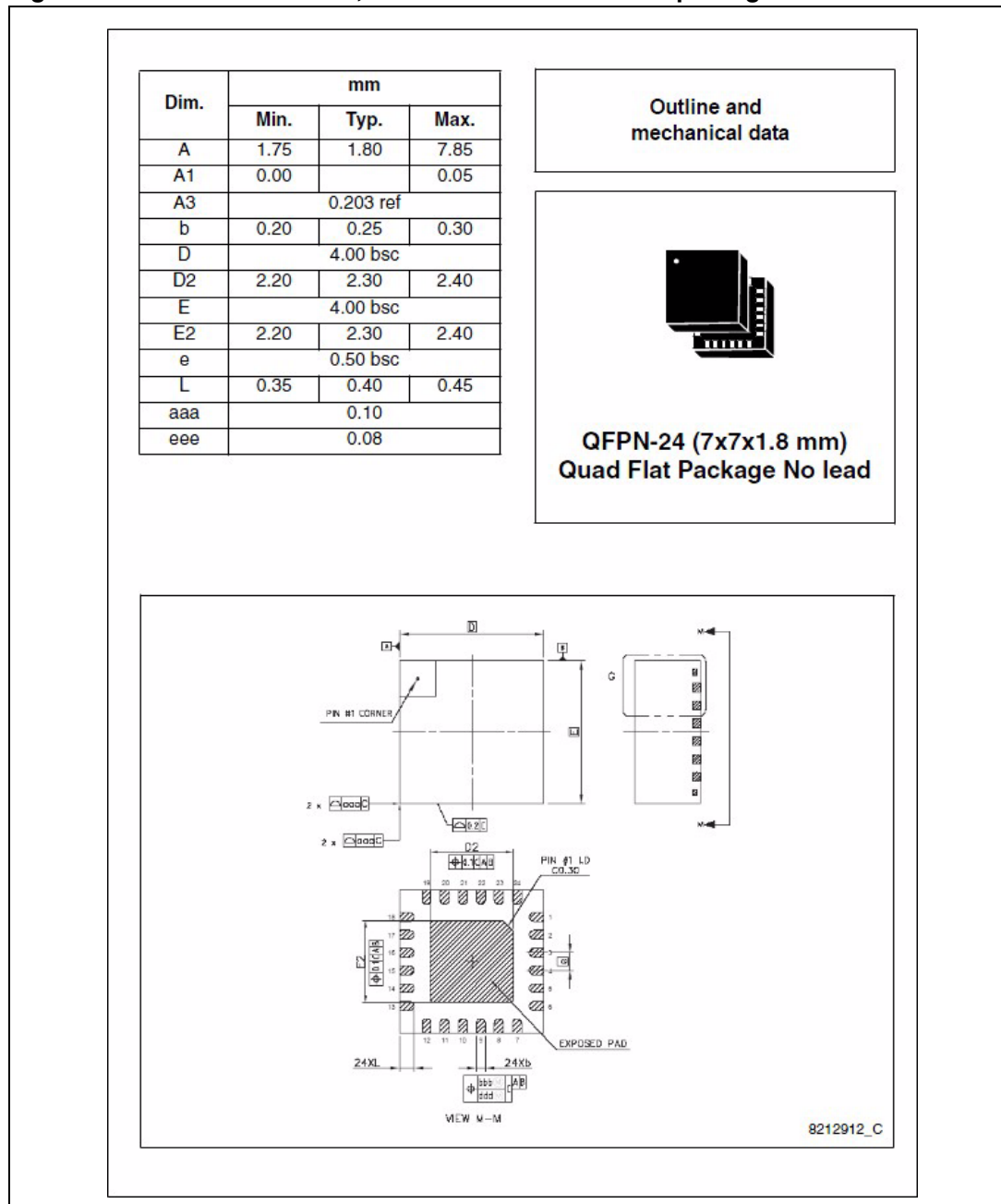
Figure 12. QFPN 4x4x1.8mm, 24L: mechanical data and package dimensions
