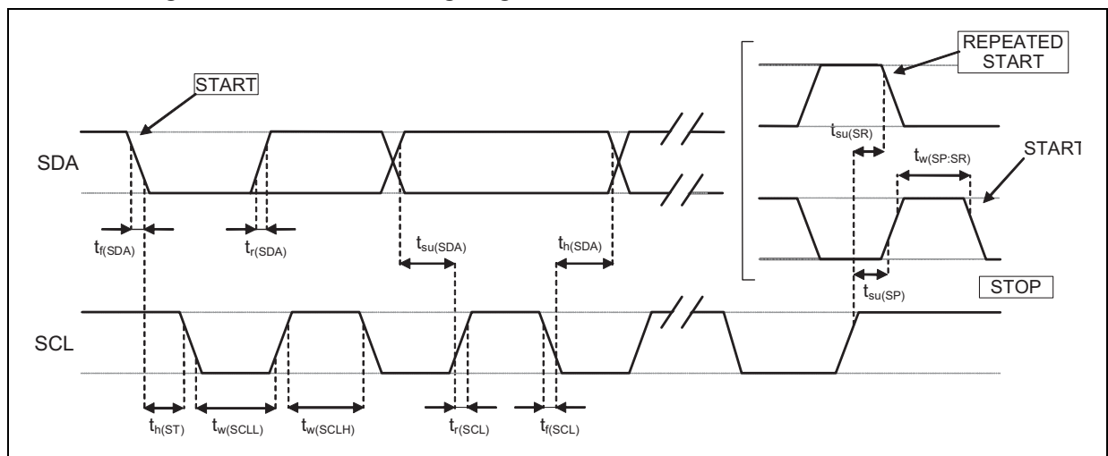
Figure 4. I 2 C Slave timing diagram (a)
