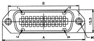
DIP TYPE FEMALE
