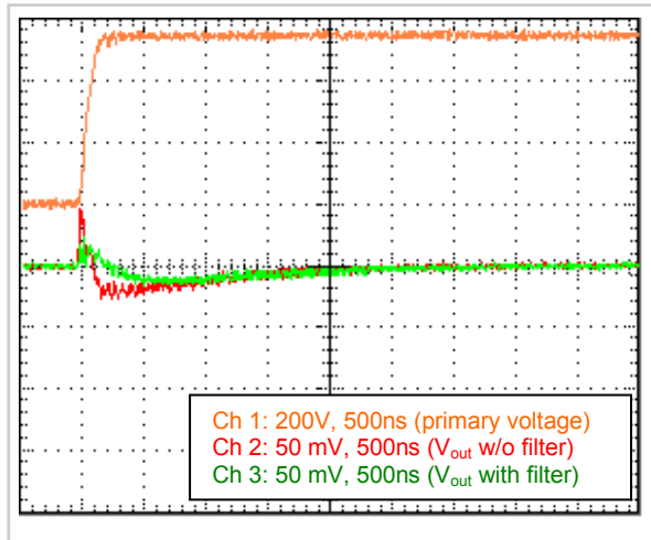
Fig. 4: dV/dt (3.7kV/ \mu s; 530V primary voltage; filter configuration acc. to Tab. 1)
