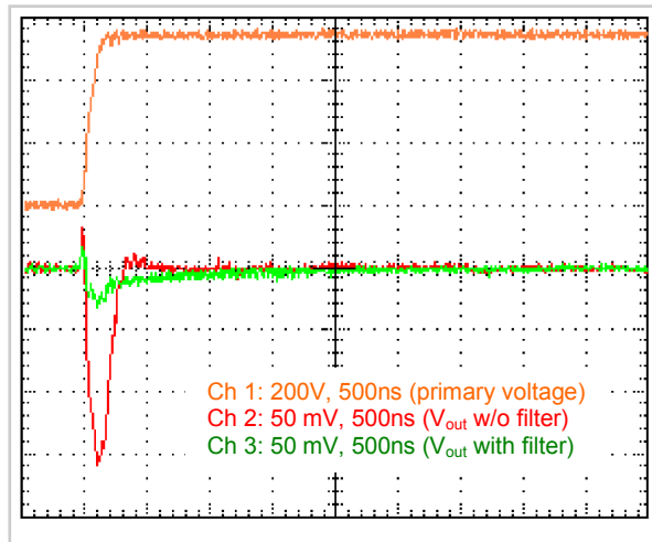
Fig. 3: dV/dt (3.7kV/ \mu s; 530V voltage on primary conductor; filter configuration acc. to Tab. 1)
