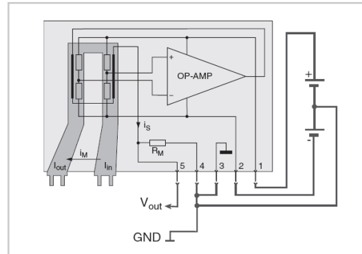
Fig. 7: Pinning of CMS3050.
