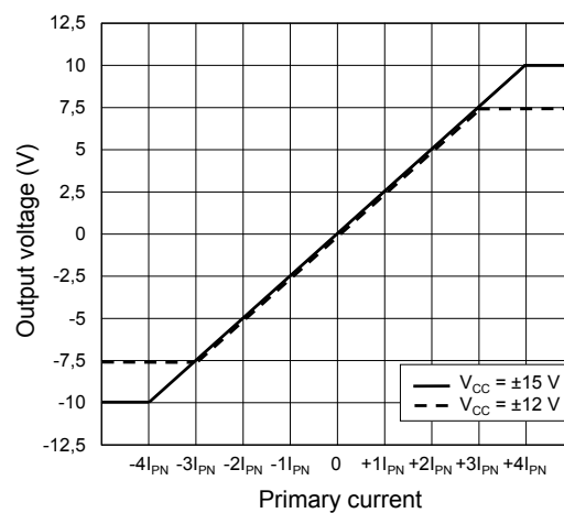
Fig. 1: Output voltage range for different supply voltages
