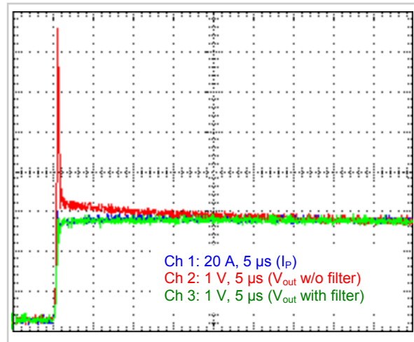
Fig. 5: Step response ( I_P = 50\text{A} ; di/dt \approx 170\text{ A}/\mu\text{s} ; filter configuration acc. to Tab. 1)
