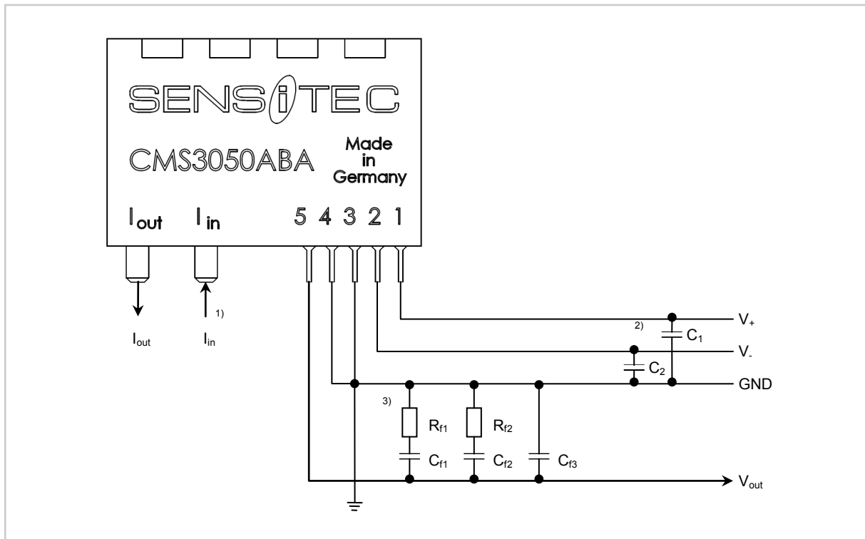
Fig. 9: Typical circuit to improve frequency response using a RC-filter network.
