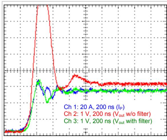
Fig. 4: Step response I_P = 50\text{A} ; di/dt \approx 400\text{ A}/\mu\text{s} ; filter configuration acc. to Tab. 1)
