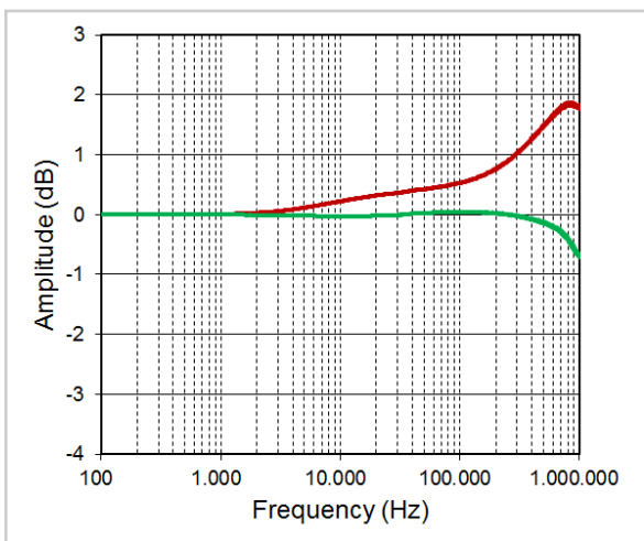
Fig. 6: Typical frequency response with RC-filter (green) and without (red). Filter configuration acc. to Tab. 1.
