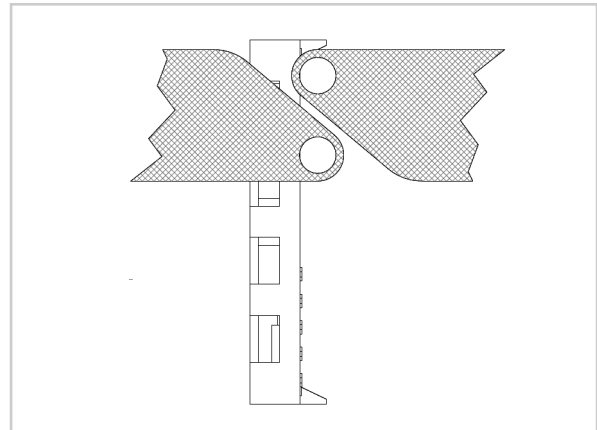
Fig. 11: Recommended current feed layout.
