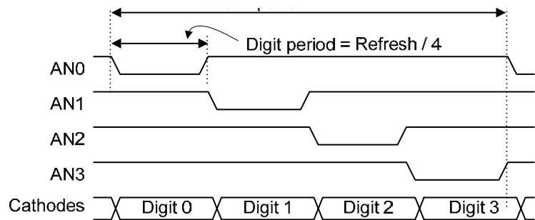
Figure 8. Multiplexed 7seg display timing
