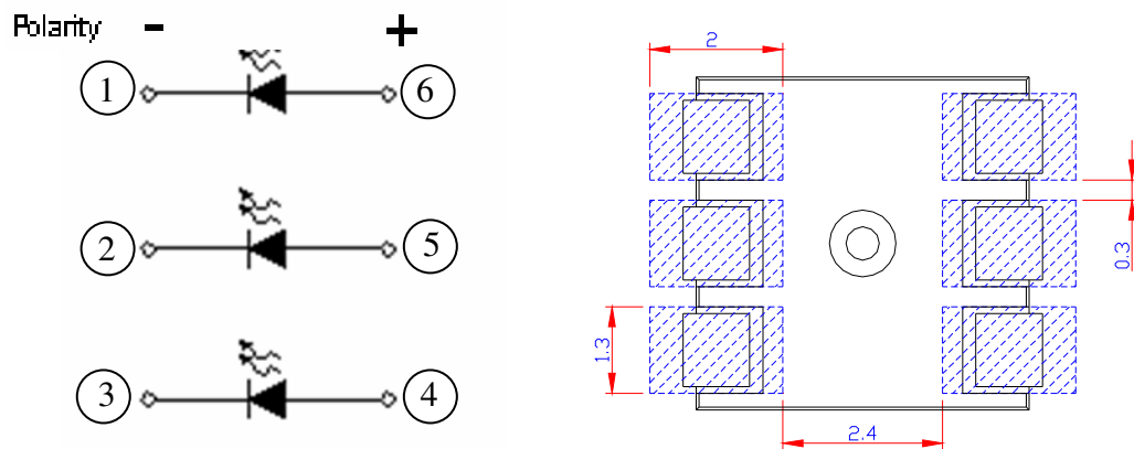
< Figure 1 PLCC 5050 series dimensions >
