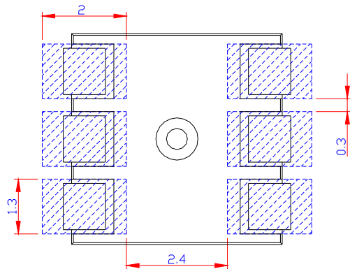
<Figure 9 Pad dimensions >
