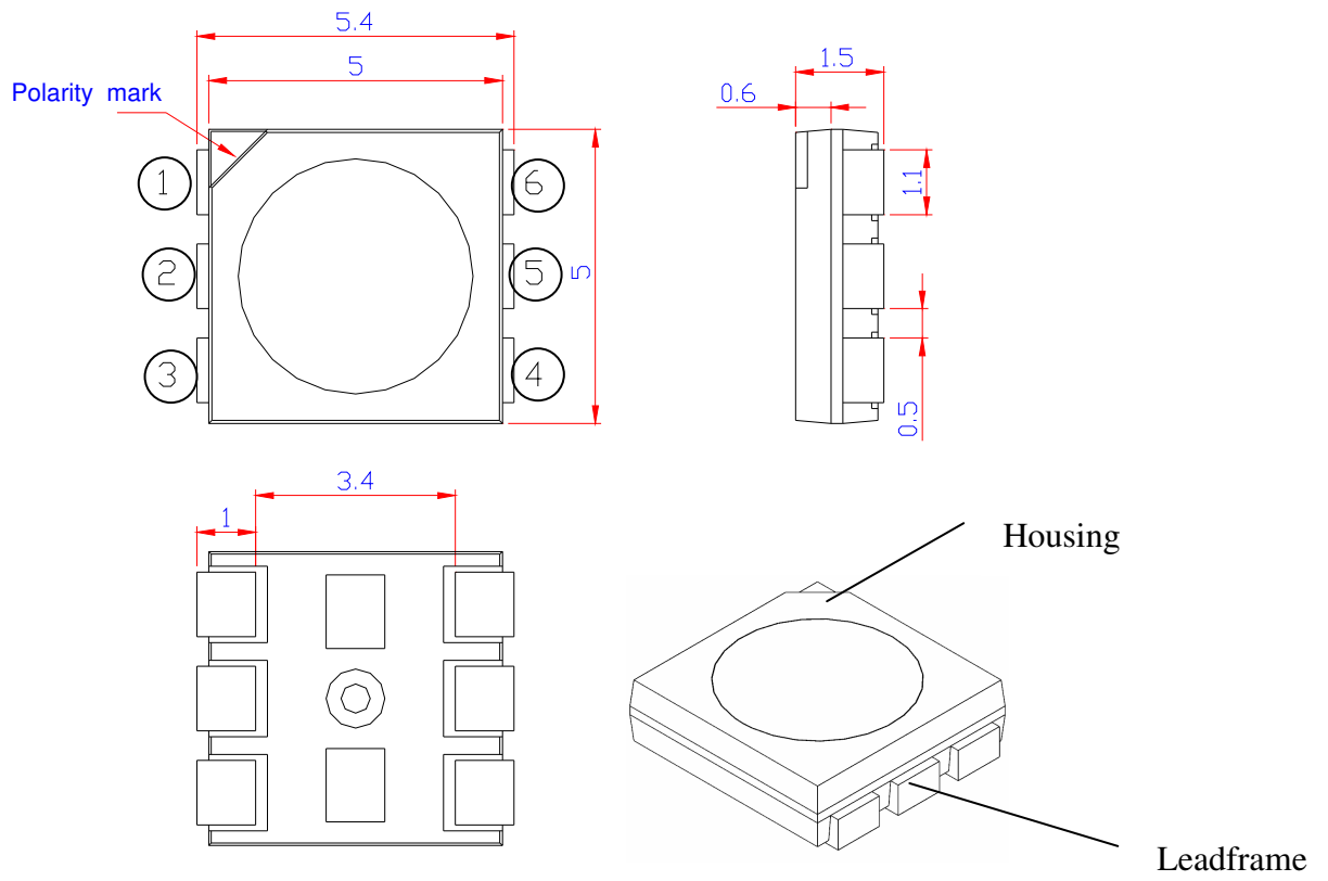
< Figure 1 PLCC 5050 series dimensions >
