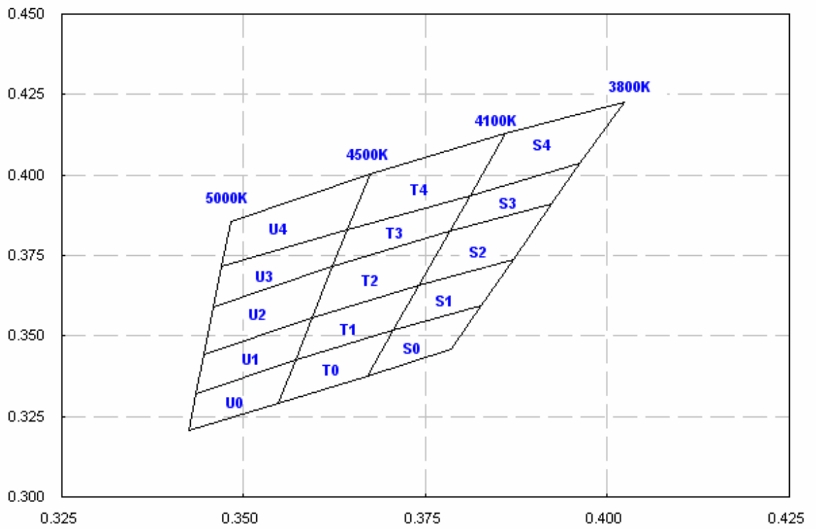
< Figure 14 PLCC 5050 series chromaticity diagram >
