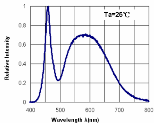
< Figure 4 Wavelength & relative intensity for PLCC 5050 series.>
