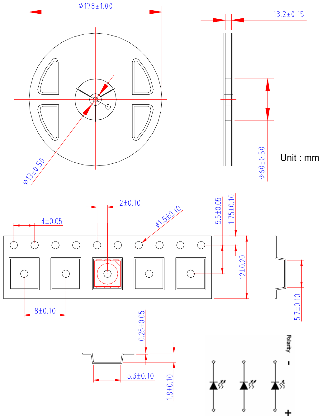
< Figure 11 Taping reel dimensions >
