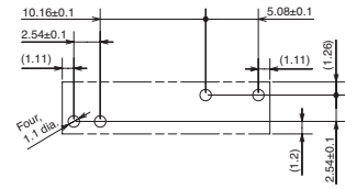
Mounting Holes (Bottom View)
