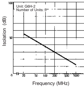
Frequency vs. Isolation
