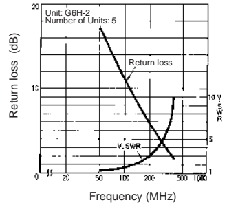
Frequency vs. Return Loss, V.SWR
