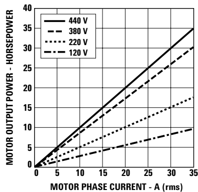
Figure 20. Motor Output Horsepower vs. Motor Phase Current and Supply Voltage.
