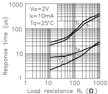
Fig.8 Response Time vs. Load Resistance
