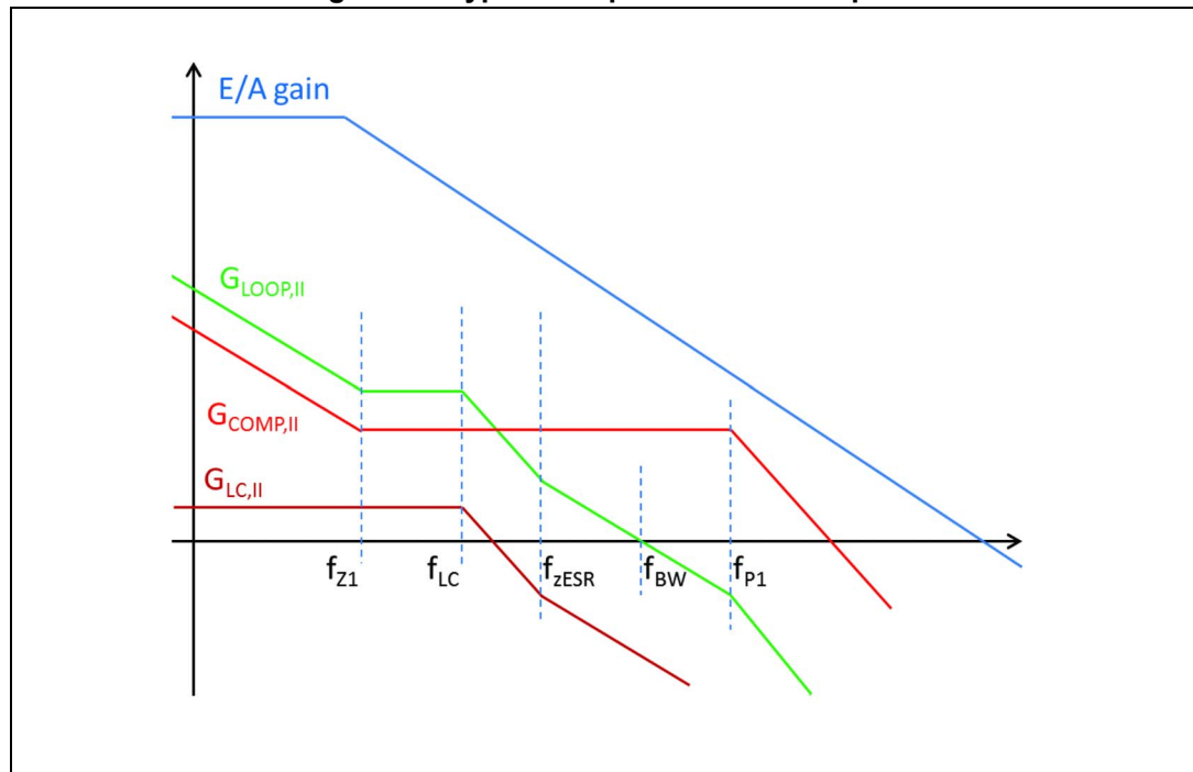
Figure 12. Type II compensation - bode plot
