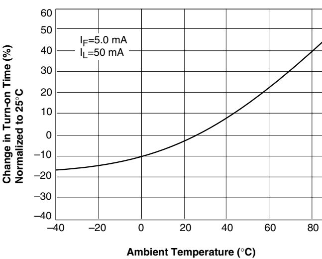
Figure 15. Turn-on Time vs. Temperature
