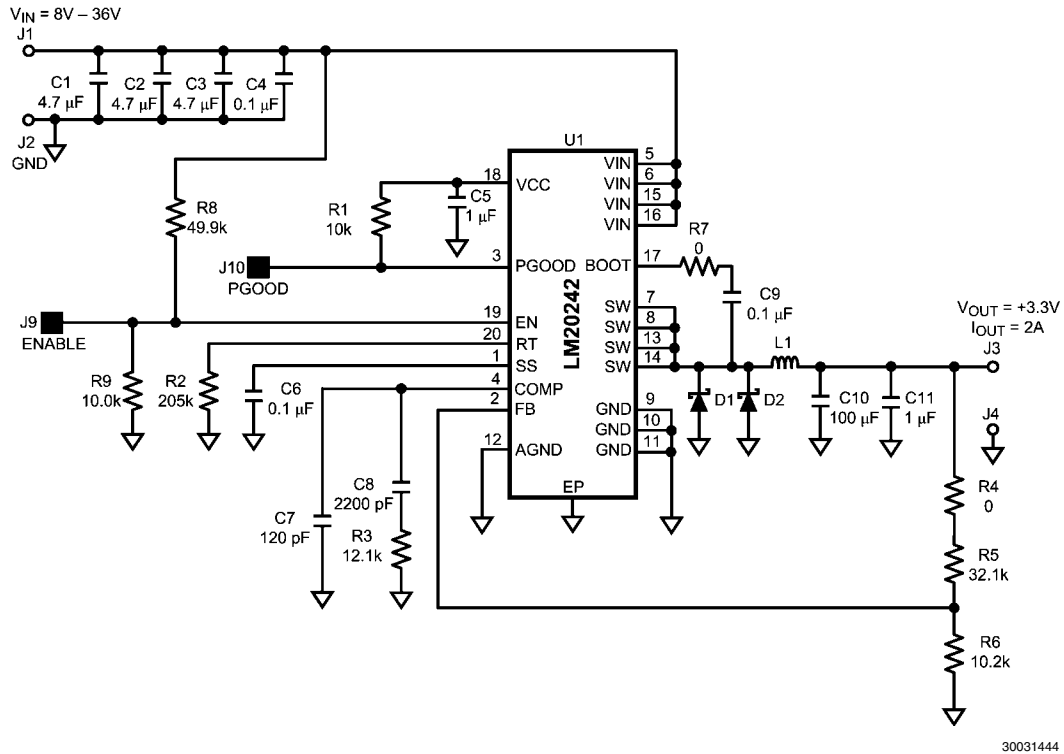
FIGURE 10. Typical Application Schematic
