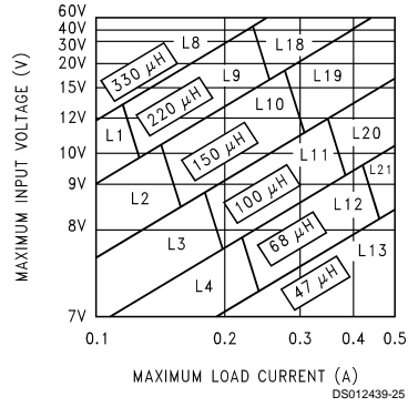
FIGURE 5. LM2594/LM2594HV-5.0
