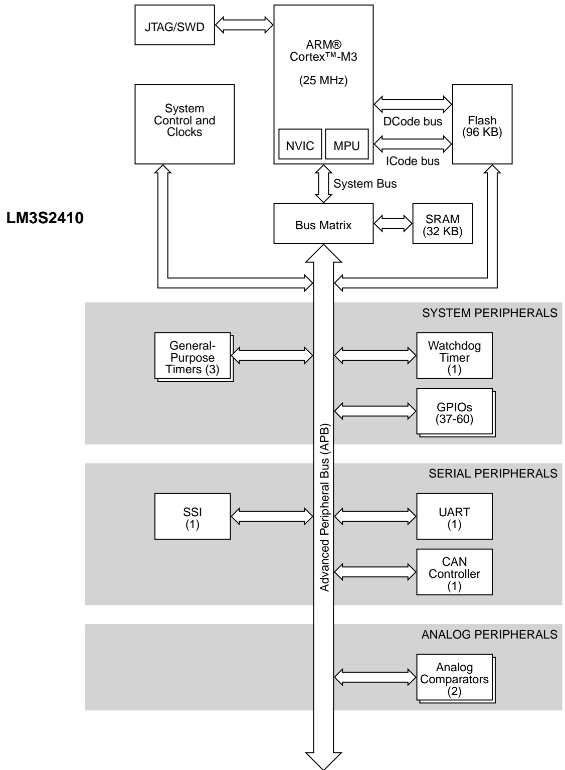
Figure 1-1. Stellaris LM3S2410 Microcontroller High-Level Block Diagram
