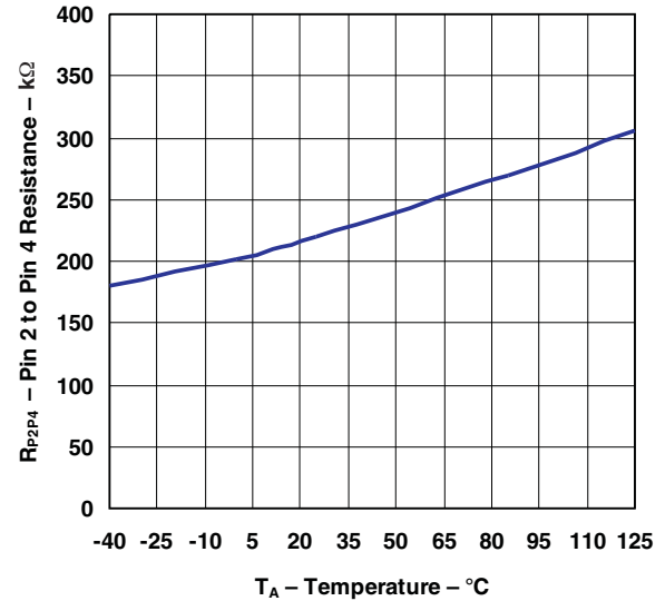
LP2951 DIVIDER RESISTANCE VS TEMPERATURE
