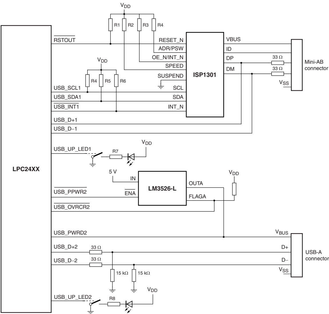
Fig 12. LPC2468 USB OTG port configuration: USB port 1 OTG dual-role device, USB port 2 host
