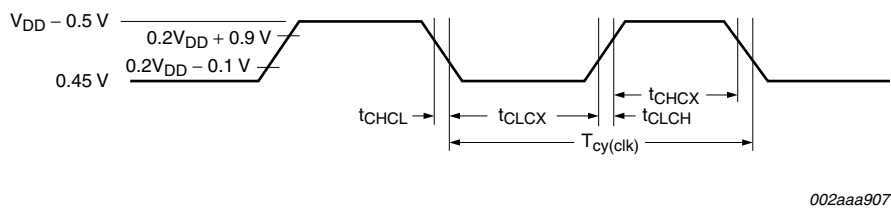
Fig 7. External clock timing
