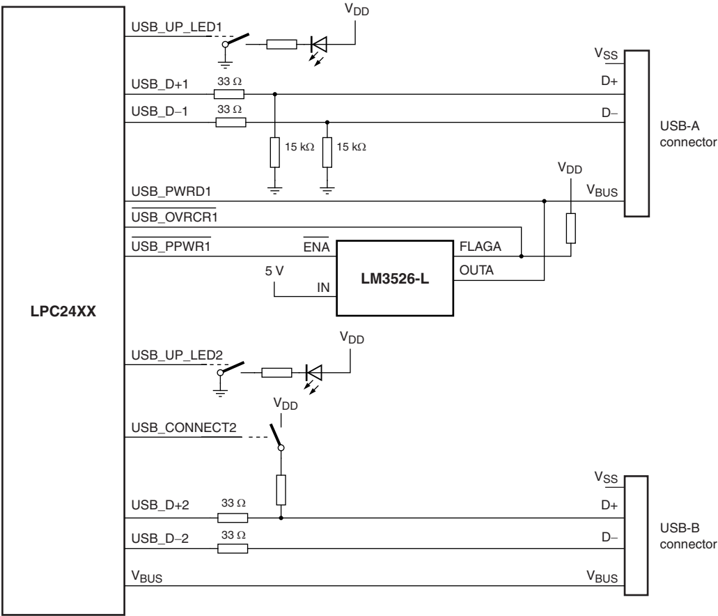
Fig 14. LPC2468 USB OTG port configuration: USB port 2 device, USB port 1 host
