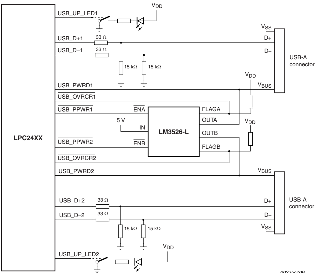
Fig 15. LPC2468 USB OTG port configuration: USB port 1 host, USB port 2 host
