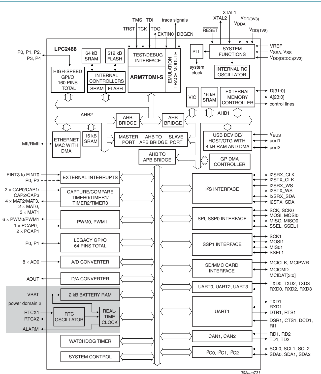
Fig 1. LPC2468 block diagram
