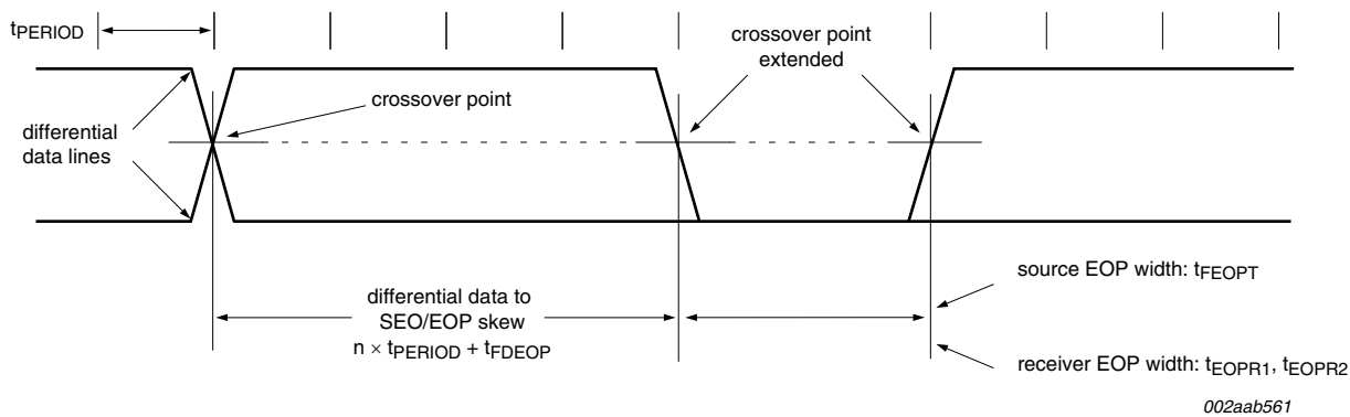
Fig 8. Differential data-to-EOP transition skew and EOP width
