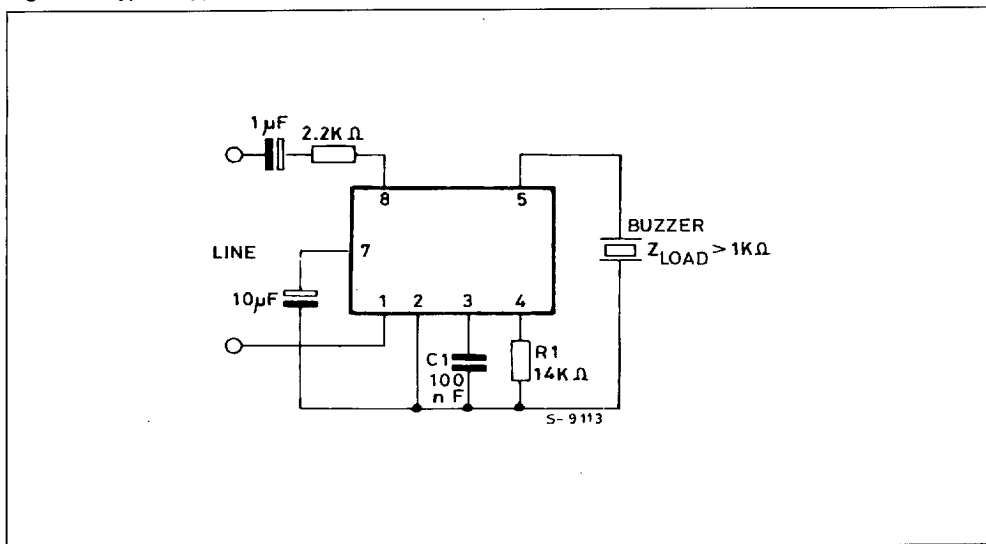
Figure 3 : Typical Application for LS1240A only.
