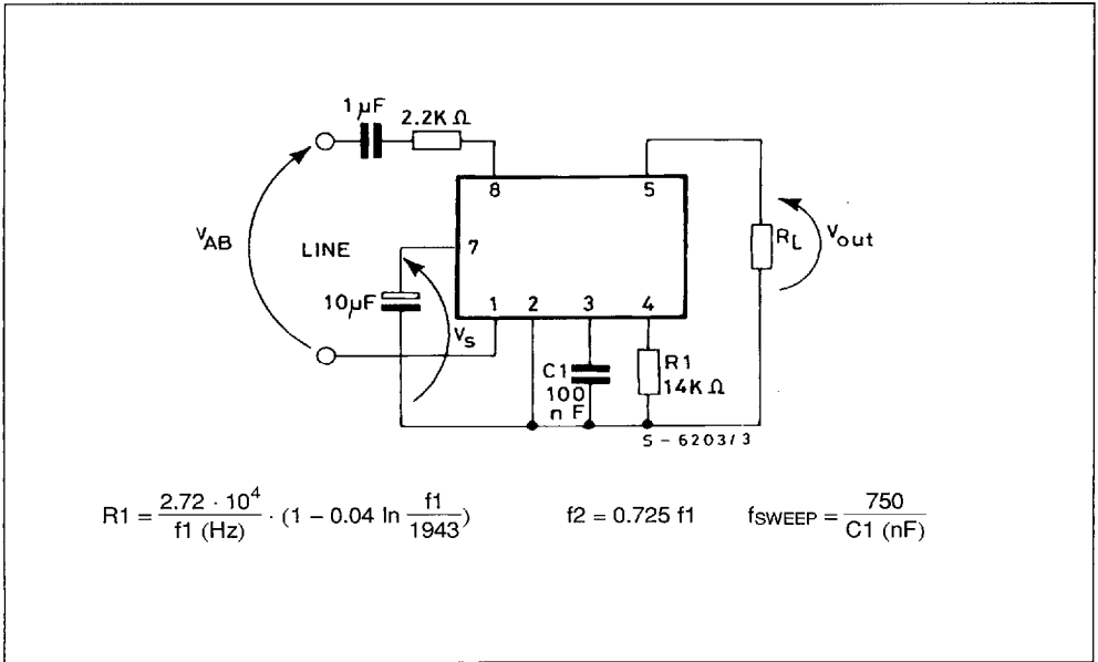
Figure 1 : Test Circuit.
