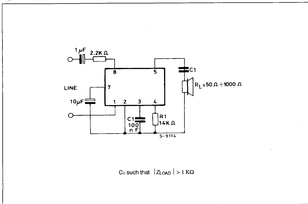
Figure 3 : Typical Application for LS1240A only.
