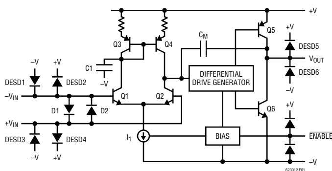
Figure 1. Simplified Schematic
