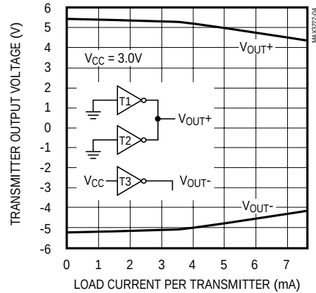
Figure 4a. MAX3241 Transmitter Output Voltage vs. Load Current per Transmitter
