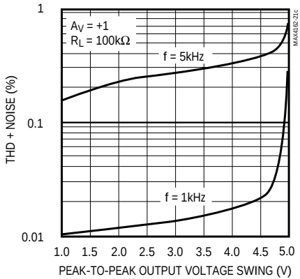
TOTAL HARMONIC DISTORTION PLUS NOISE vs. OUTPUT VOLTAGE SWING
