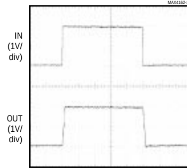
NONINVERTING LARGE-SIGNAL PULSE RESPONSE ( V_{DD} = 3V , C_L = 0pF )
