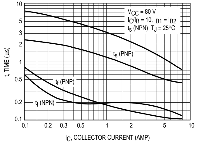
Figure 10. Turn-Off Times
