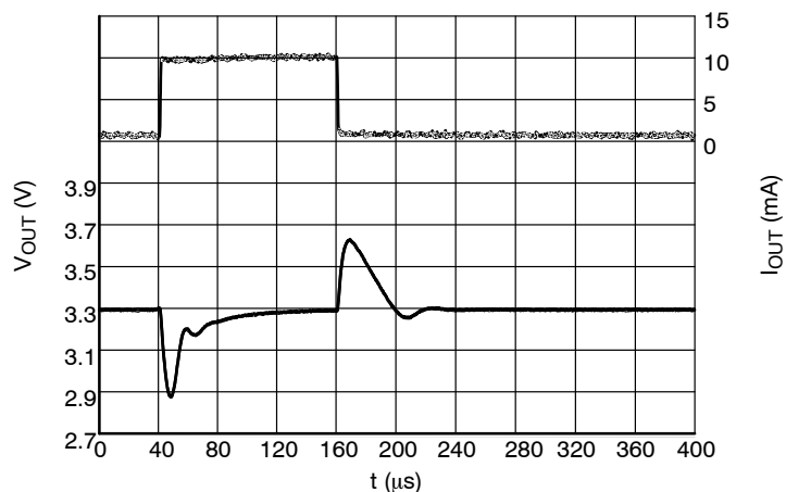
Figure 28. Load Transients, 3.3 V Version, Load Step 1 mA to 10 mA, V_{IN} = 4.3 \text{ V}
