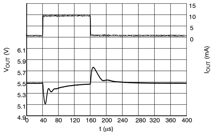
Figure 29. Load Transients, 5.5 V Version, Load Step 1 mA to 10 mA, V_{IN} = 6.5 \text{ V}
