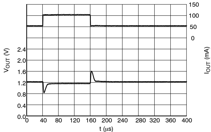
Figure 30. Load Transients, 1.2 V Version, Load Step 50 mA to 100 mA, V_{IN} = 2.5 \text{ V}
